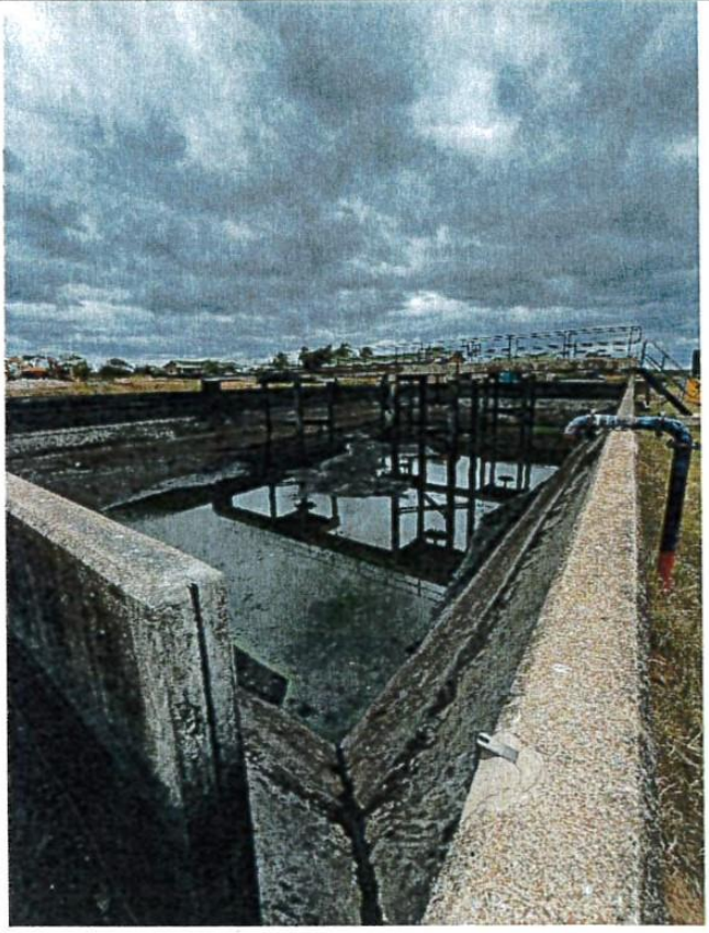
Dewatering of existing BNR
