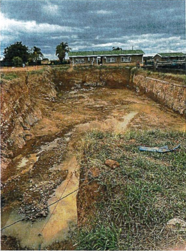
Excavation of new BNR
